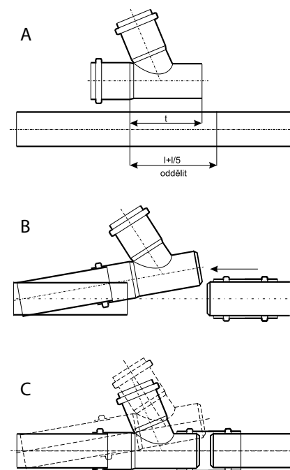
Figure 6 Subsequent connection – procedure II
